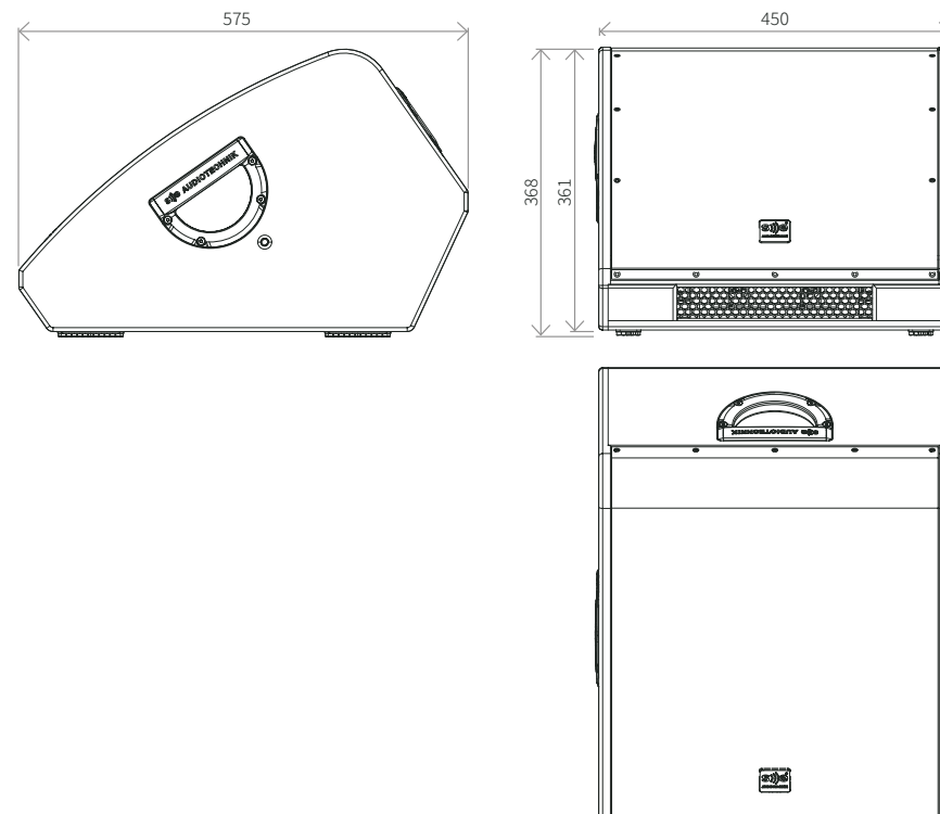
Figure 13. SMX12A views and dimensions. Annotations given in millimeters.
