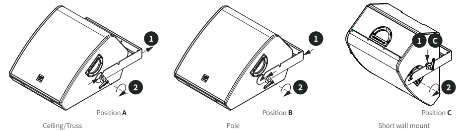
Figure 7. Different positioning options offered by the SMX 12UB U-bracket.
