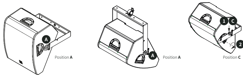
Figure 11. Different aiming angles for wall- and truss-mount installation.
