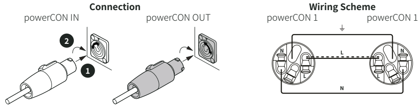
Figure 5. PowerCON® plug-in and link cable connection.
