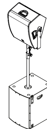
Figure 12. SMX 12A pole-mounted over an S15 subwoofer from SE AUDIOTECHNIK®.
