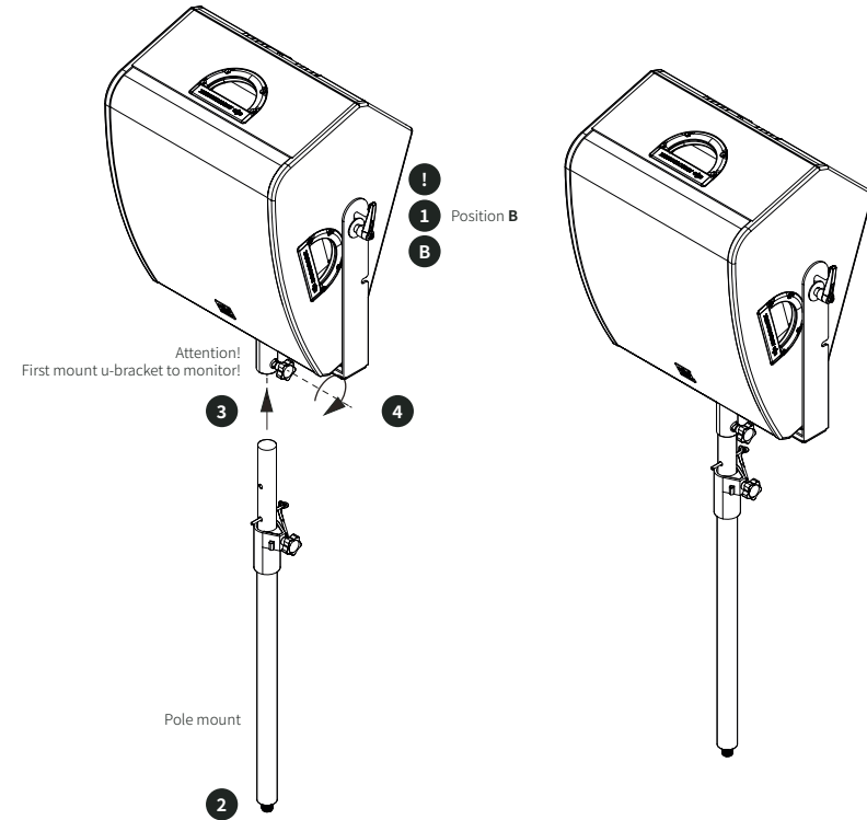
Figure 10. Mounting the SMX 12A with the U-bracket in the SPS20 pole bar.
