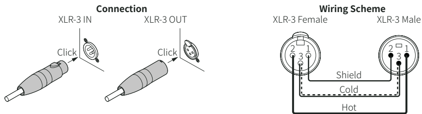
Figure 6. XLR-3 plug-in and link cable connection.
