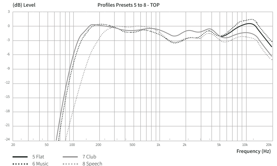
Figure 16. Profile curves of the TOP presets.
