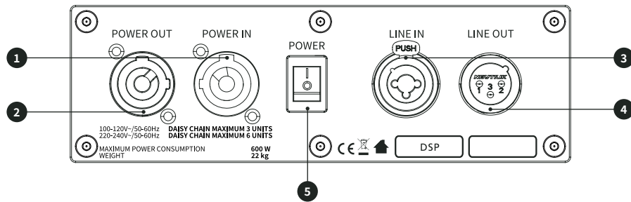
Figure 3. SMX 12A input panel.
