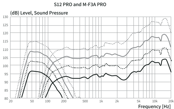
Figure S1. SPL generated by different combinations of S12 PRO subwoofers and M-F3A PRO units.
