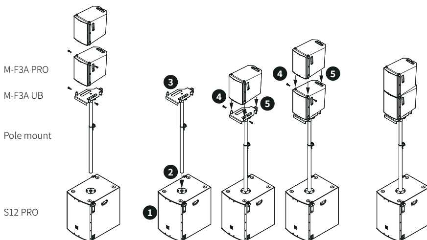
Figure 9. Installation of small arrays with a pole mount and the M-F3A UB U-bracket.
