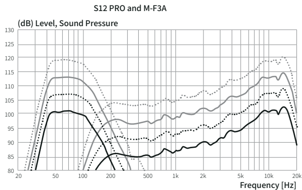
Figure S2. SPL generated by different combinations of S12 PRO subwoofers and M-F3A units.
