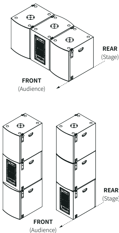
Figure 54. Some configurations for Cardioid setups.
