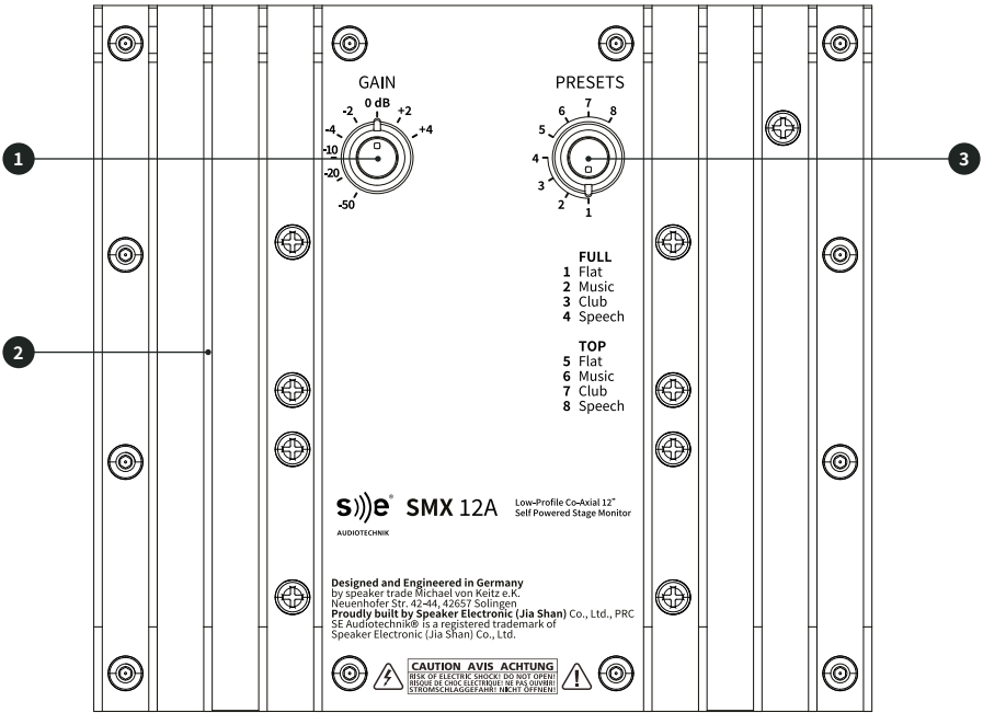
Figure 2. SMX 12A amplifier panel.
