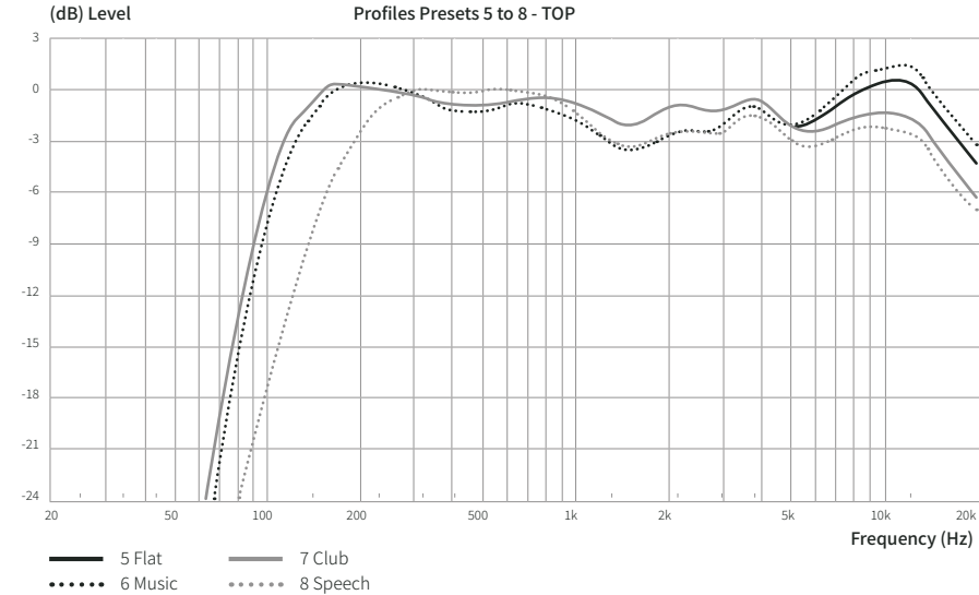
Figure 16. Profile curves of the TOP presets.
