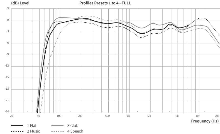
Figure 15. Profile curves of the FULL presets.
