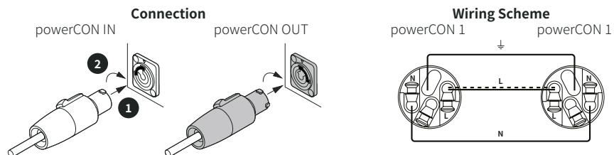
Figure 5. PowerCON® plug-in and link cable connection.
